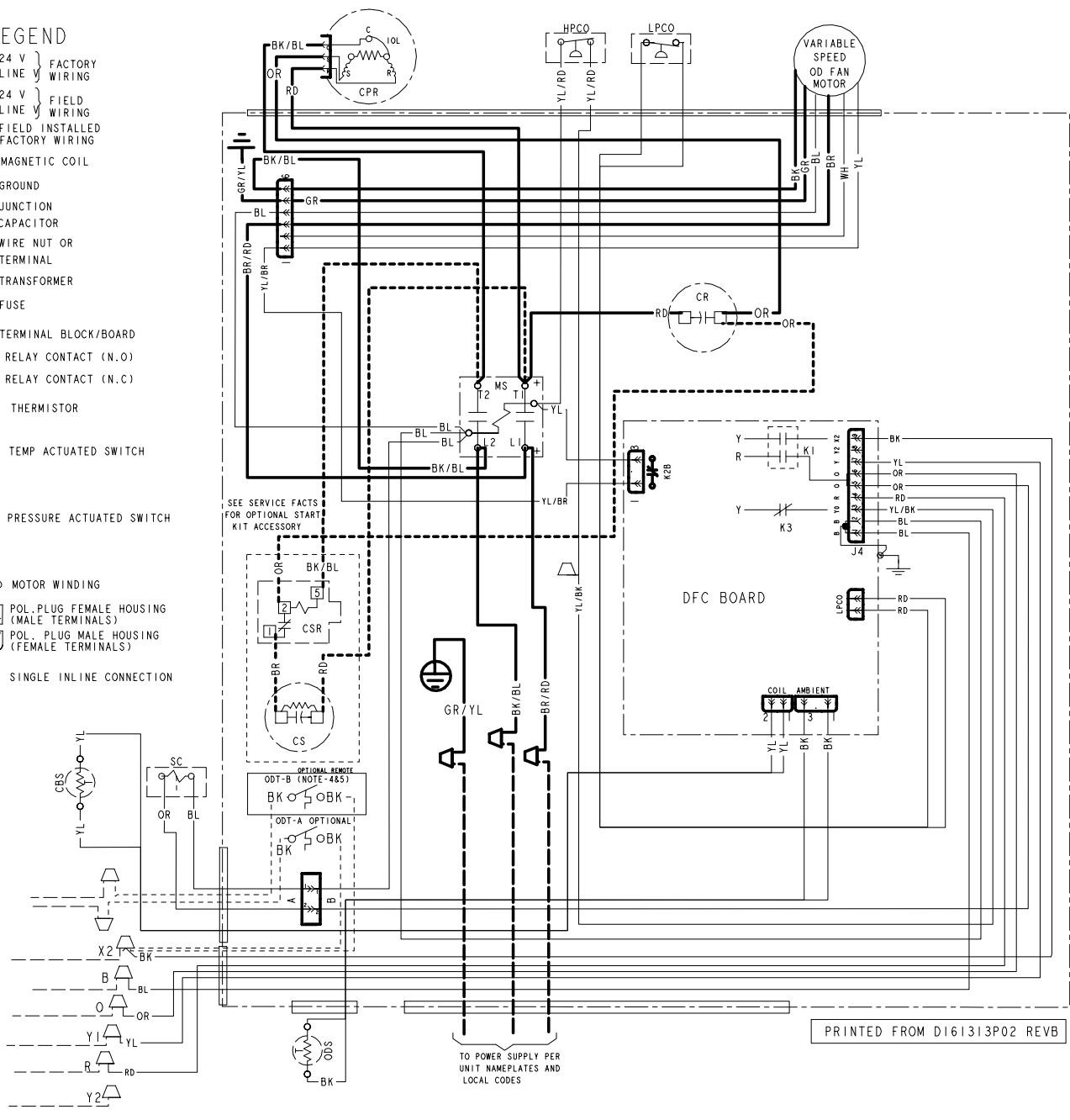
Figure 2. 3.5 Ton Model
