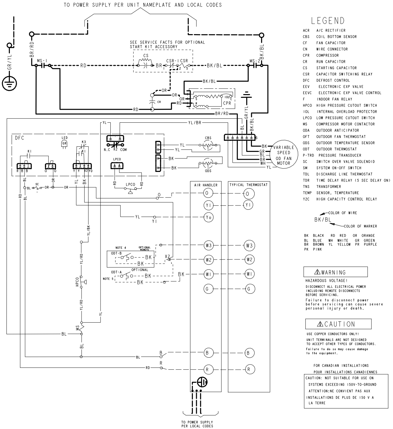
Figure 1. 3.5 Ton Model
